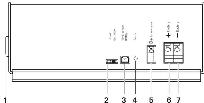
Fig. 1: Connections
