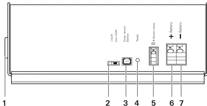
Fig. 1 : Raccordements
