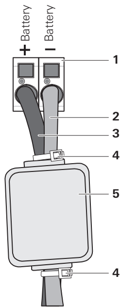
Fig. 3: Snap ferrite
