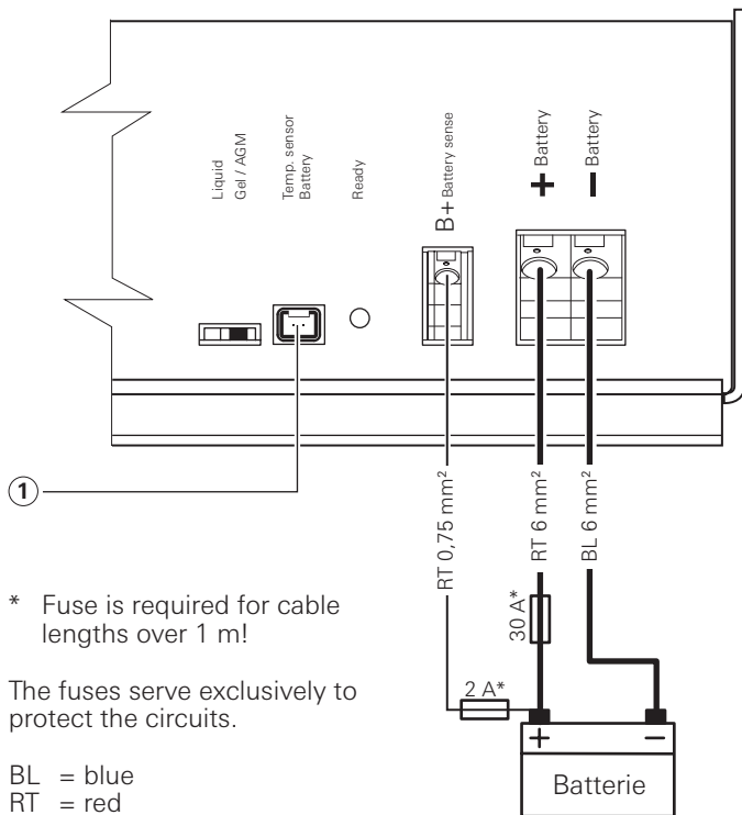
Fig 4: Wiring diagram
